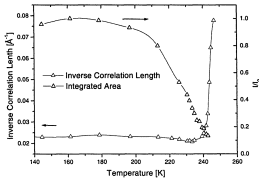
Figure 1 : Temperature dependence of the integrated intensity, and inverse correlation length of the (4.667, 0, 5) CO superlattice peak.
