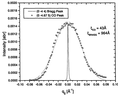
Figure 2 : Longitudinal scan through the (0,-4,4) and (0,-4.66, 5) Bragg and charge order peaks
